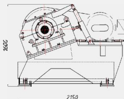
Granulator M 500 / 620
