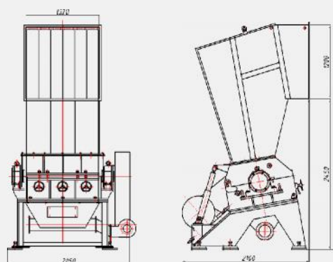
Granulator M 600 / 1200
