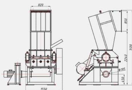
Granulator M 500 / 800
