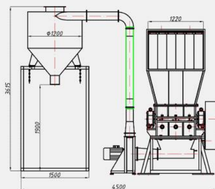
Granulator M 500 / 800 with module
